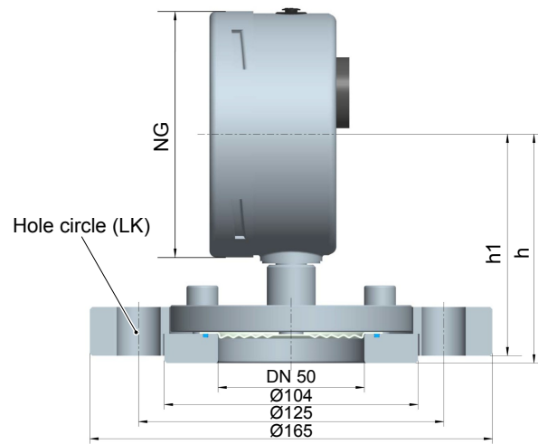
Fig. 6: Collar flange
